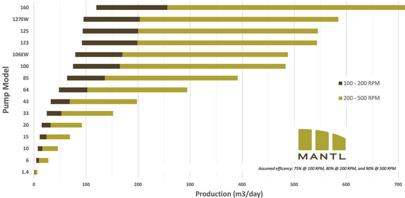
Pump Model vs. Production (m3/day) High Speed 100 - 500 RPM
